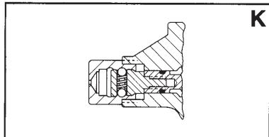
K 2K, 2-Position Detented Cap 3K, 3-Position Detented Cap
