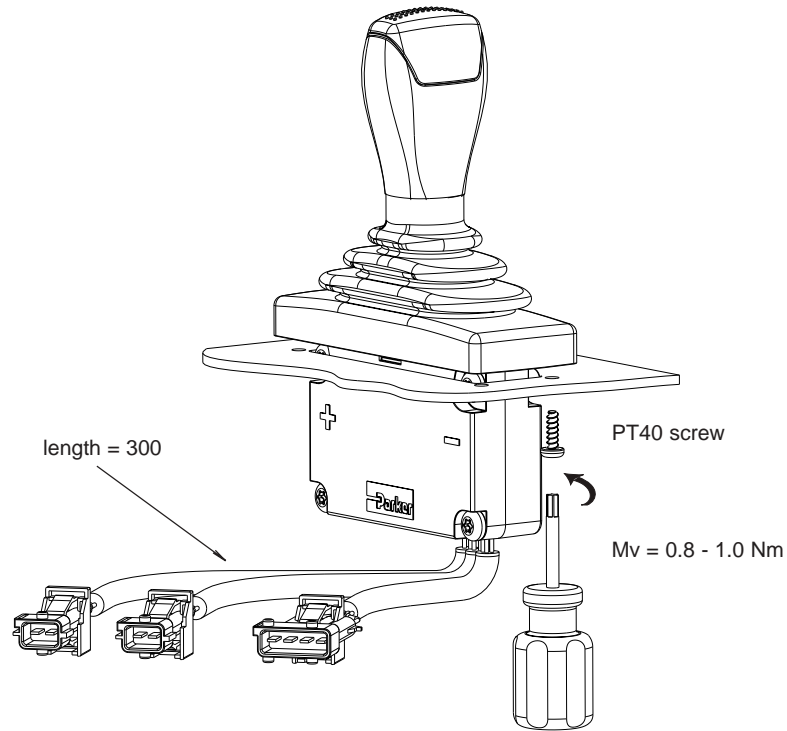
Maximum screw engagement
