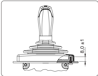
Maximum screw engagement
